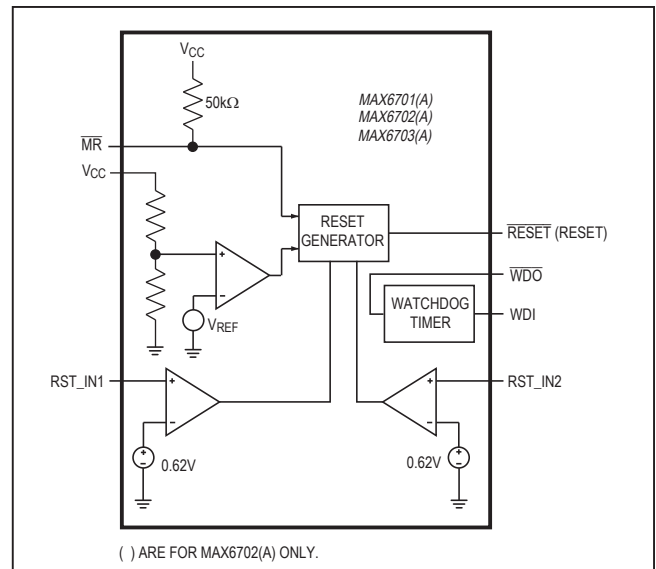
Figure 3. MAX6701(A)/MAX6702(A)/MAX6703(A) Functional Diagram
