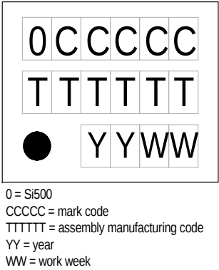
Figure 2. Top Mark
