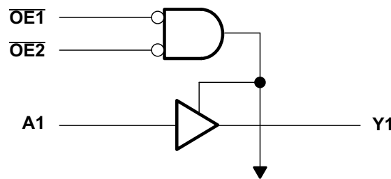
To Seven Other Channels Simplified Schematic
