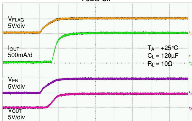
Power On
