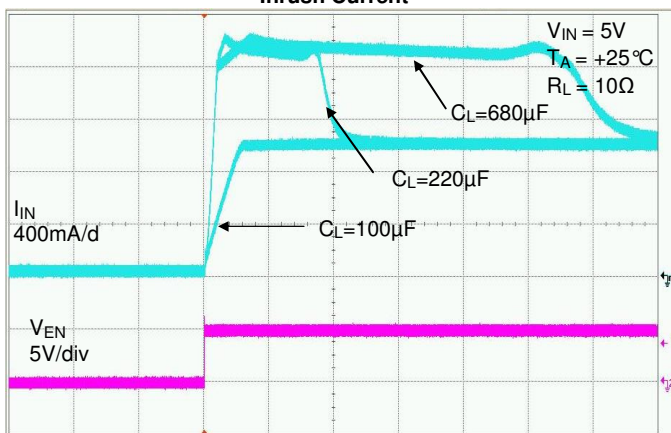
Inrush Current
