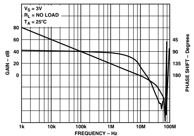
TPC 18. Open-Loop Gain and Phase vs. Frequency
