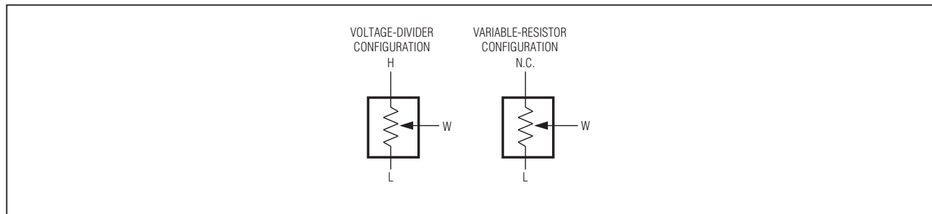
Figure 1. Voltage-Divider/Variable-Resistor Configurations
