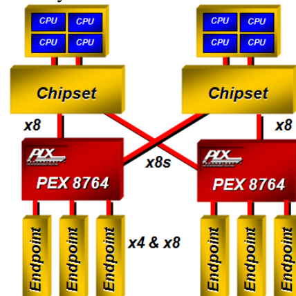
Figure 9. Host Fail-Over
