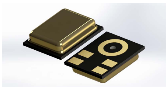
RHLGA metal cap 5-lead 3.5 x 2.65 x 0.98 mm
