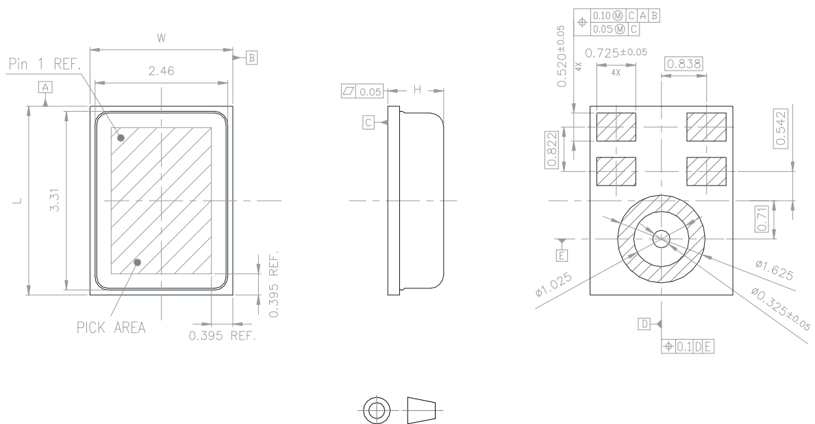
Figure 5. RHLGA metal cap 5-lead (3.5 x 2.65 x 0.98 mm) package outline and mechanical data
