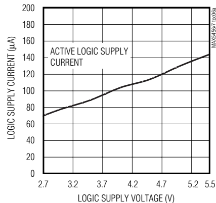
LOGIC SUPPLY CURRENT vs. LOGIC SUPPLY VOLTAGE
