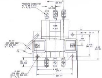
3 POLE Weight 3.0 lbs.
