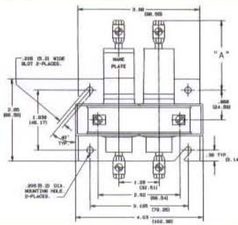
2 POLE Weight 2.0 lbs.
