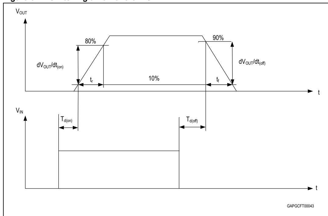
Figure 5. Switching time waveforms
