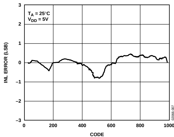
Figure 7. AD5316 INL
