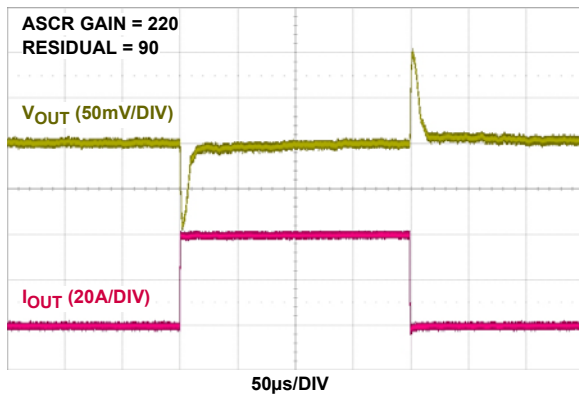
FIGURE 12. 5V IN TO 1V OUT TRANSIENT RESPONSE, f_{SW} = 571kHz , C_{OUT} = 8 \times 100\mu F CERAMIC + 4x470 \mu F POSCAP
