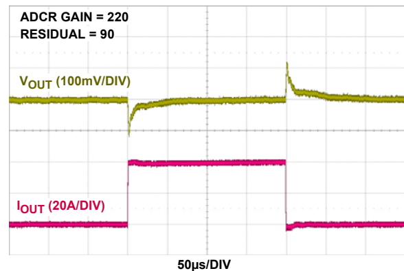
FIGURE 17. 12V IN TO 2.5V OUT TRANSIENT RESPONSE, f_{SW} = 800kHz , C_{OUT} = 6 \times 100\mu F CERAMIC + 3x470 \mu F POSCAP
