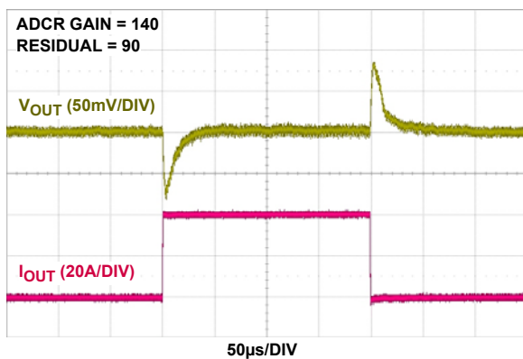
FIGURE 14. 12V IN TO 1V OUT TRANSIENT RESPONSE, f_{SW} = 300kHz , C_{OUT} = 14 \times 100\mu F CERAMIC + 6x470 \mu F POSCAP
