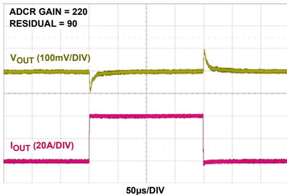
FIGURE 16. 12V IN TO 1.5V OUT TRANSIENT RESPONSE, f_{SW} = 571kHz , C_{OUT} = 10 \times 100\mu F CERAMIC + 4x470 \mu F POSCAP
