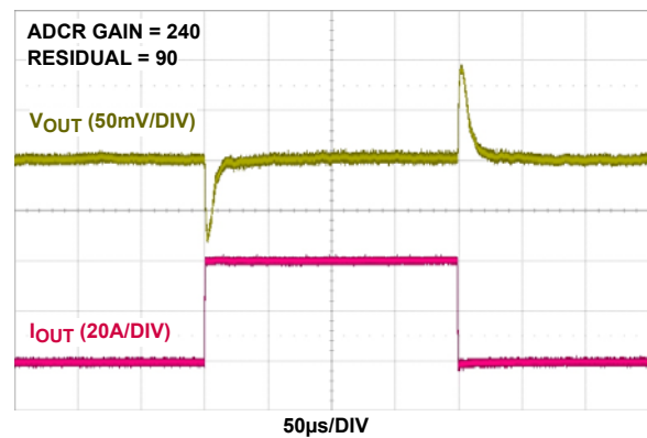
FIGURE 15. 12V IN TO 1V OUT TRANSIENT RESPONSE, f_{SW} = 571kHz , C_{OUT} = 10 \times 100\mu F CERAMIC + 4x470 \mu F POSCAP
