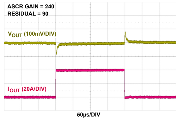
FIGURE 13. 5V IN TO 1.5V OUT TRANSIENT RESPONSE, f_{SW} = 571kHz , C_{OUT} = 10 \times 100\mu F CERAMIC + 4x470 \mu F POSCAP
