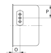
Connection style -07, 3 to 20A types (same dimensions as style -06)
