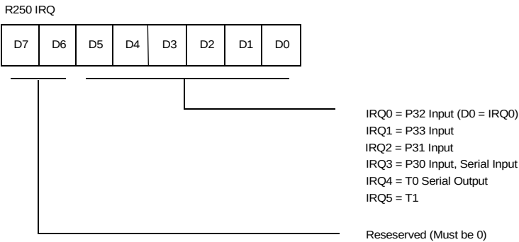
Figure 38. Interrupt Request Register (FAH: Read/Write)
