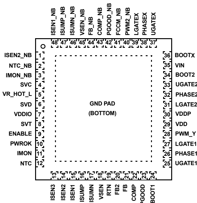
ISL6277 (48 LD QFN) TOP VIEW
