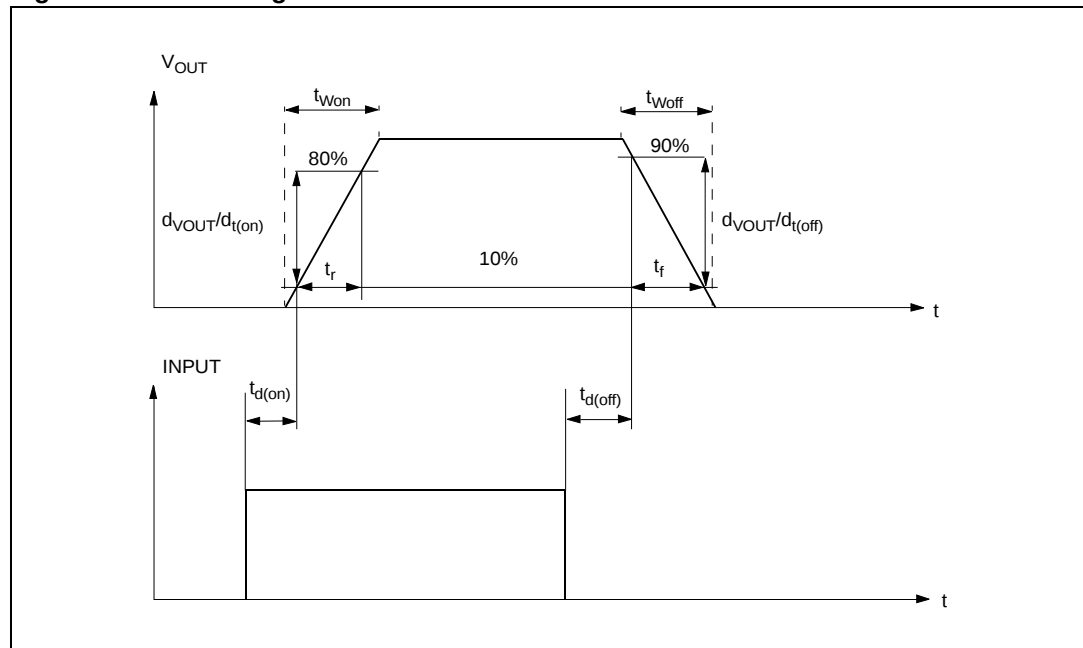
Figure 5. Switching characteristics
