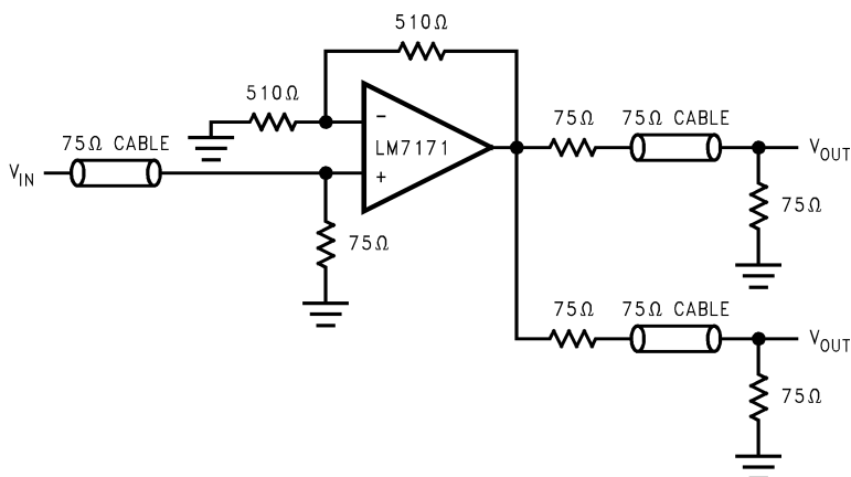
Figure 66. Video Line Driver
