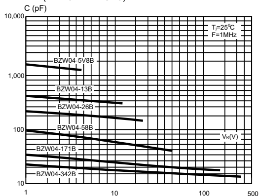
FIG.6- CHARACTERISTICS VERSUS REVERSE APPLIED VOLTAGE FOR UNIDIRECTIONAL TYPES (TYPICAL VALUES)
