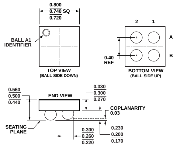
Figure 39. 4-Ball Wafer Level Chip Scale Package [WLCSP] (CB-4-5) Dimensions shown in millimeters
