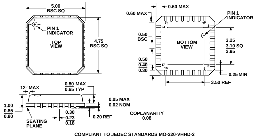
Figure 46. 32-Lead Lead Frame Chip Scale Package [LFCSP] (CP-32-2)
