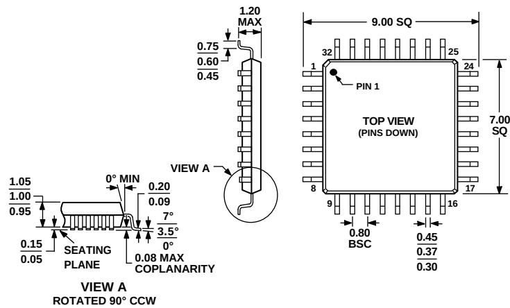
Figure 47. 32-Lead Thin Plastic Quad Flat Package [TQFP] (SU-32-2)
