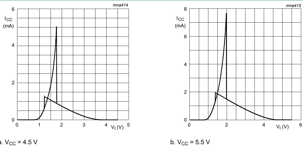
Fig. 11. Typical 74AHCT14 transfer characteristics
