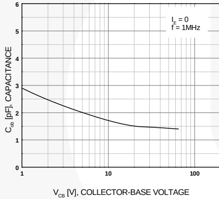
Figure 3. Output Capacitance
