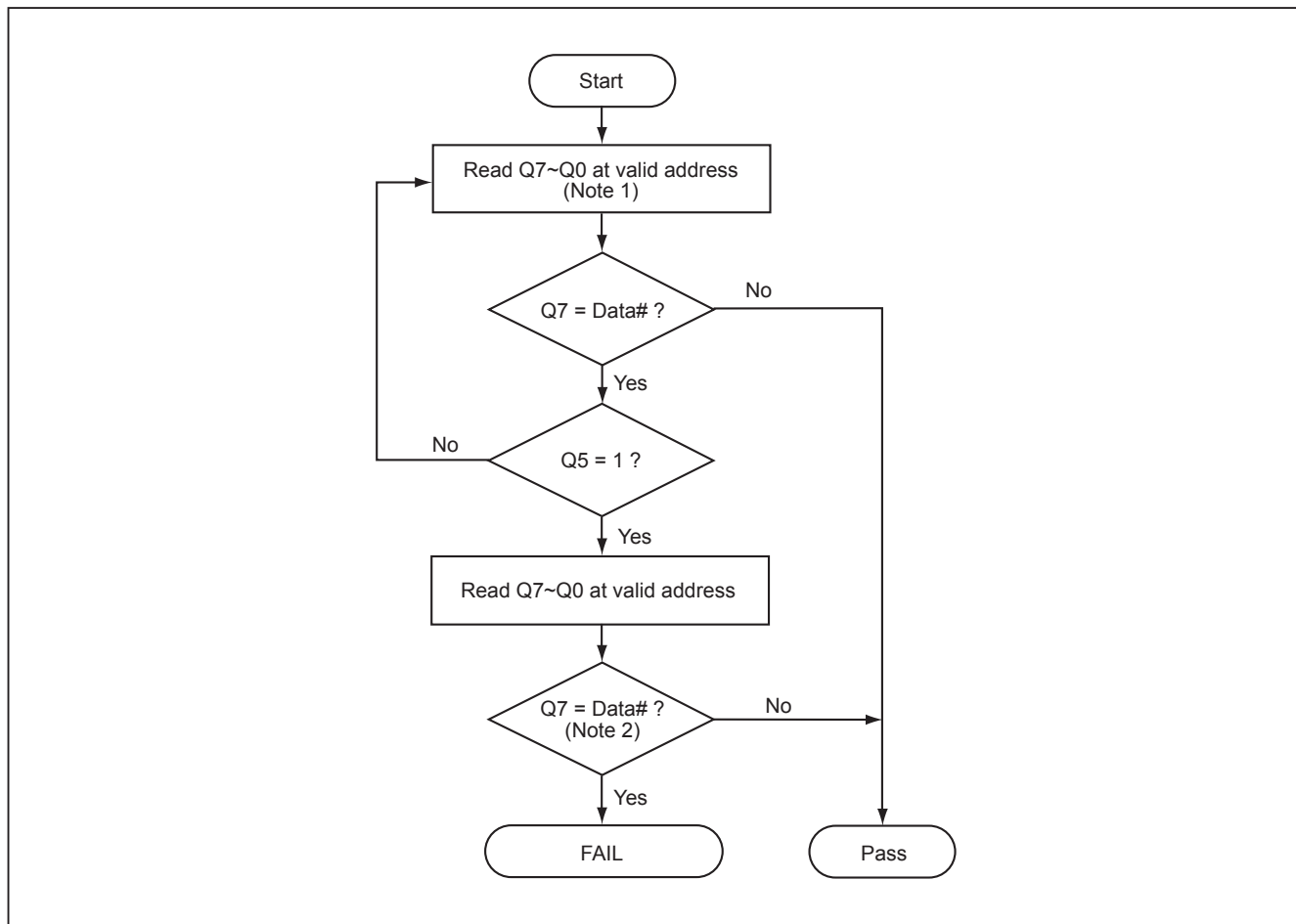
Figure 14. DATA# POLLING ALGORITHM
