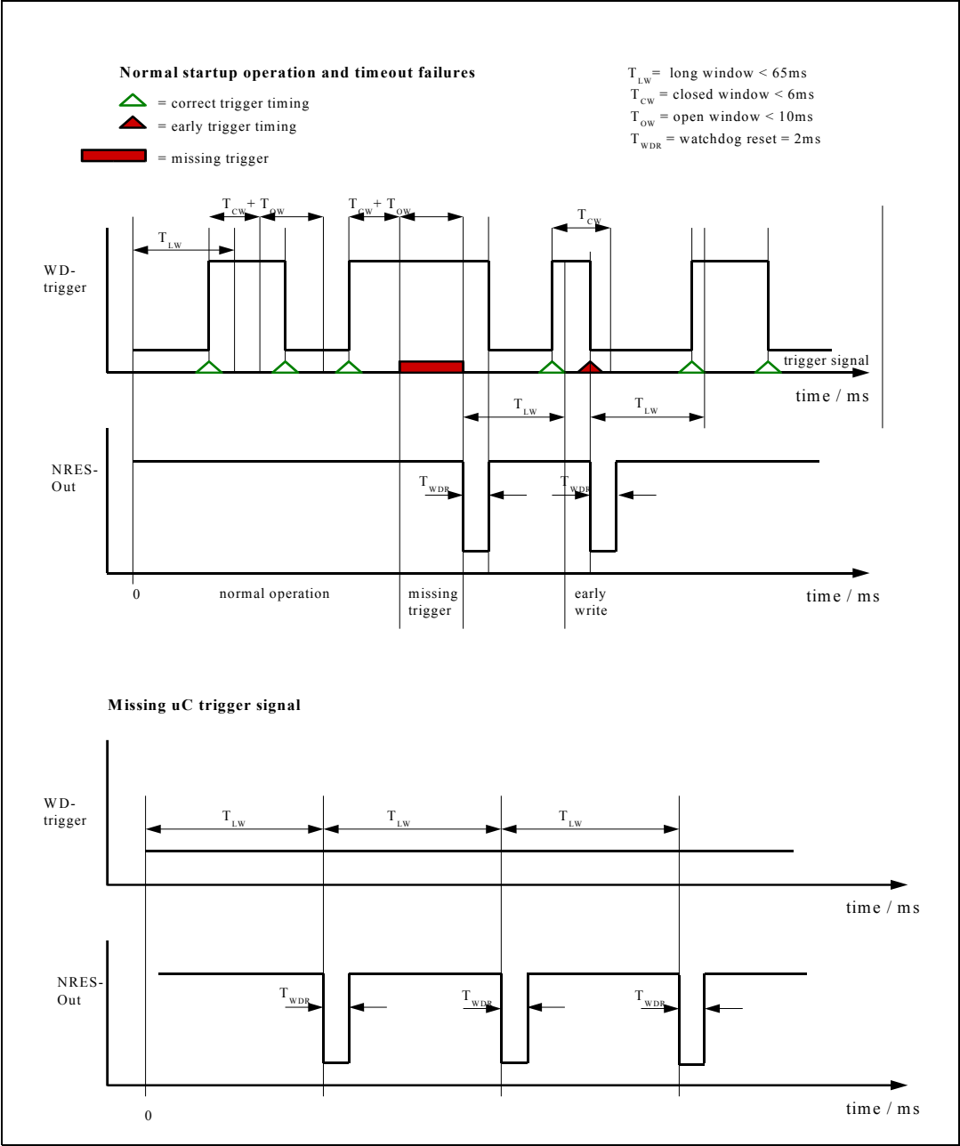
Figure 13. Watchdog timing
