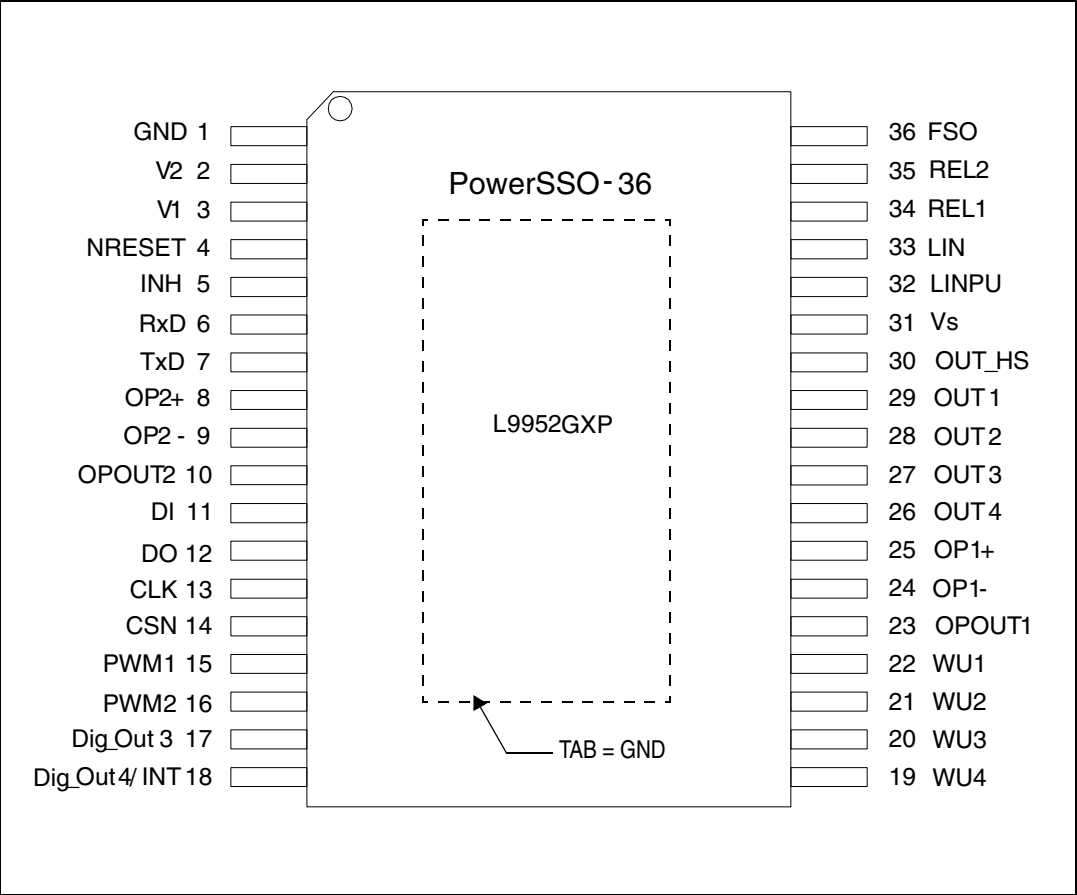
Figure 2. Pins configuration
