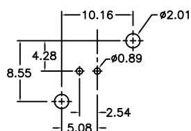
P.C. Board Layout for Type B
