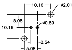
P.C. Board Layout for Type A
