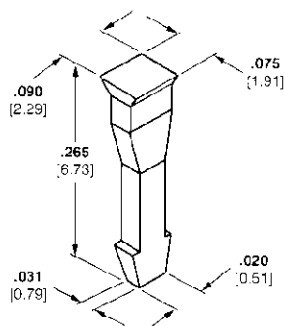
Keying Plug—Military Part No. M55302/127-00KY, AMP Part No. 102188-1
