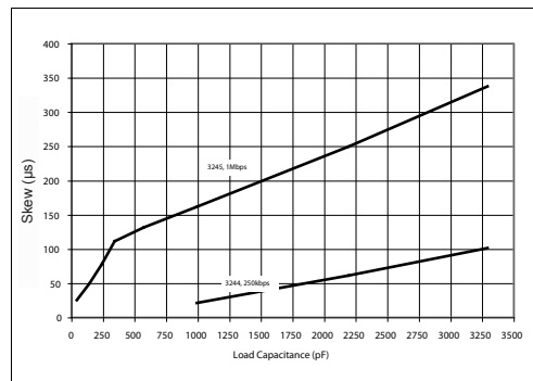
Transmitter Skew vs. Load Capacitance
