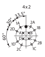
Drilling diagram for 60° indexing angle
