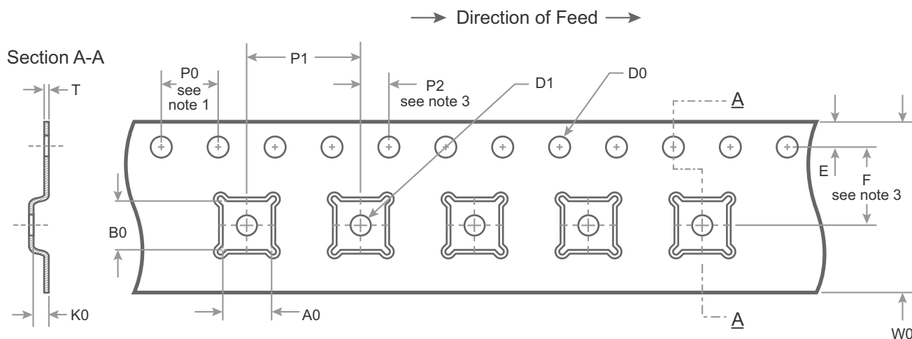
Figure 38 • Tape and Reel Specifications for 32-lead 5 \times 5 \times 0.85 mm QFN
