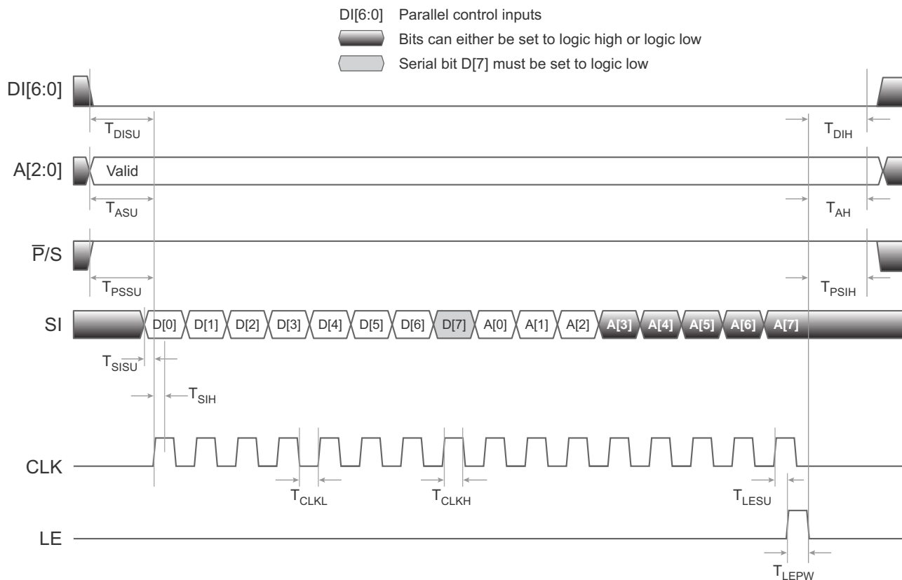
Figure 3 • Serial Timing Diagram
