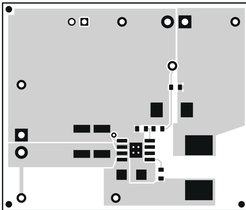
Figure 3-1. Top-Side Layout
