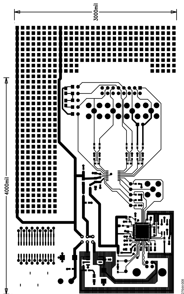
Figure 8. AD7785 Evaluation Board—Solder Side View
