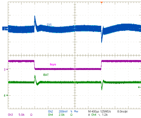
CH2: system voltage (AC), 200mV/div; CH3: system load current, 5A/div; CH4: battery charge current, 2A/div, 400us/div
