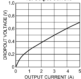
MIC2951x Dropout Voltage vs. Output Current
