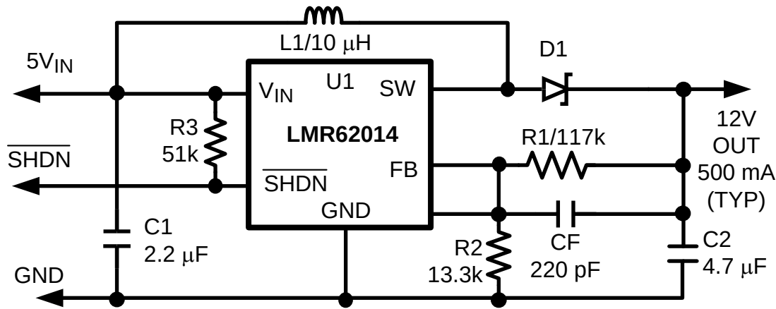
Connection Diagram
