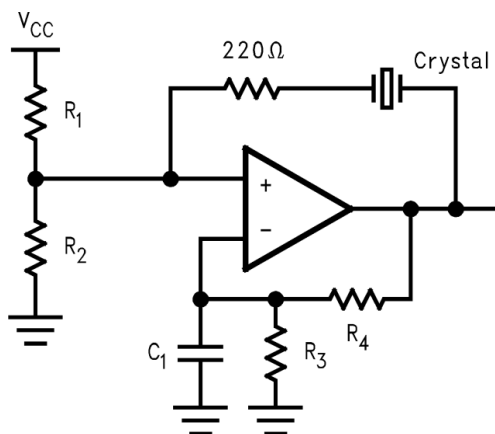
Figure 42. Crystal Oscillator
