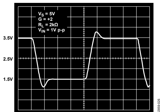
Figure 26. Large Signal Step Response; V_S = +5\text{V} , G = +2
