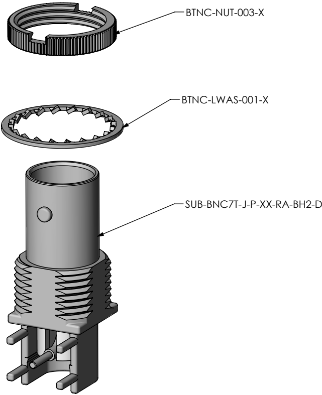
FIG. 1 BNC7T-J-P-XX-RA-BH2D SHOWN
