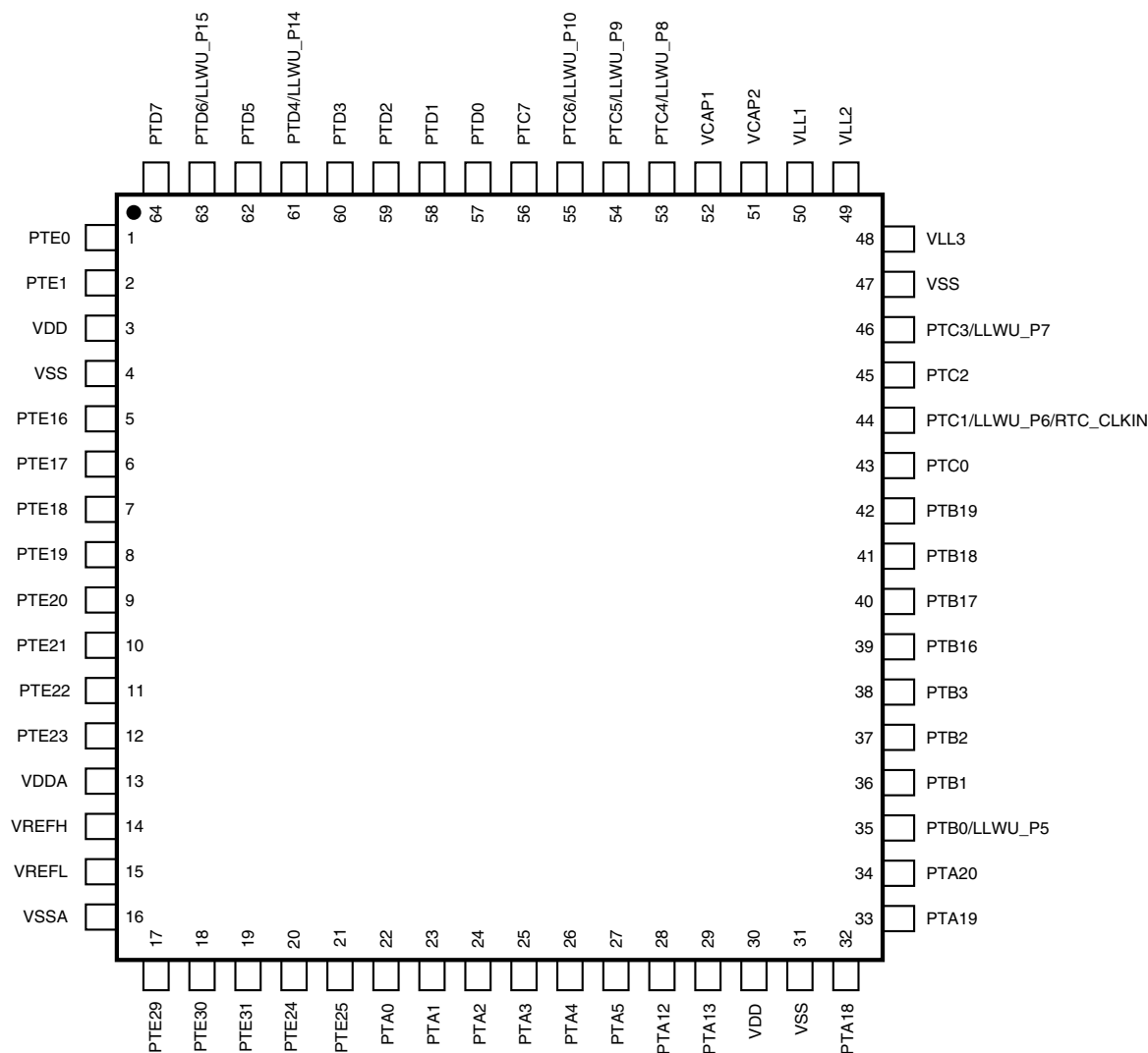
Figure 25. KL36 64-pin LQFP pinout diagram
