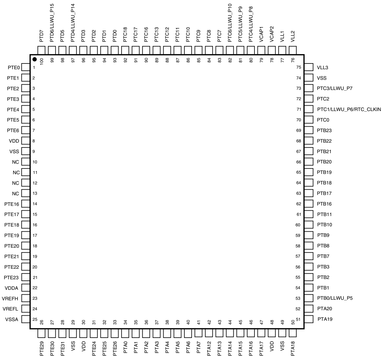
Figure 23. KL36 100-pin LQFP pinout diagram
