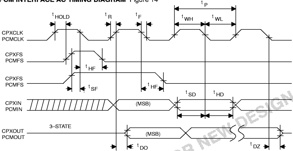
PCM INTERFACE AC TIMING DIAGRAM Figure 14
