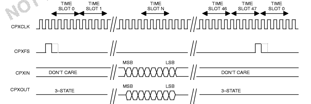
DS2130 CPX-SIDE INTERFACE Figure 8
