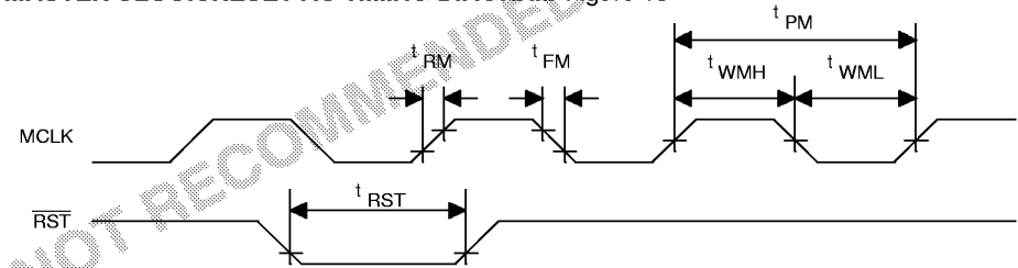
MASTER CLOCK/RESET AC TIMING DIAGRAM Figure 15
