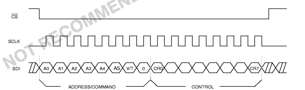
SERIAL PORT WRITE Figure 2
