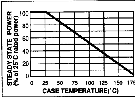
STEADY STATE POWER DERATING
