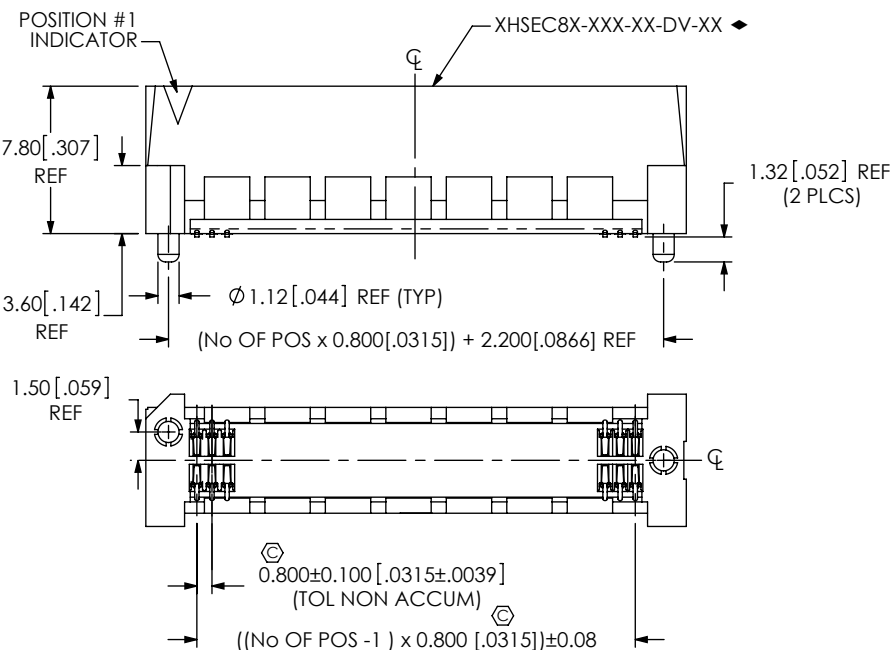
FIG 1 FOR POSITIONS -T0, -20 & -30 HSEC8-130-01-XX-DV-A SHOWN (SOME FEATURES NOT SHOWN FOR CLARITY) ◆=(SEE TABLE 9, SHT 3)
