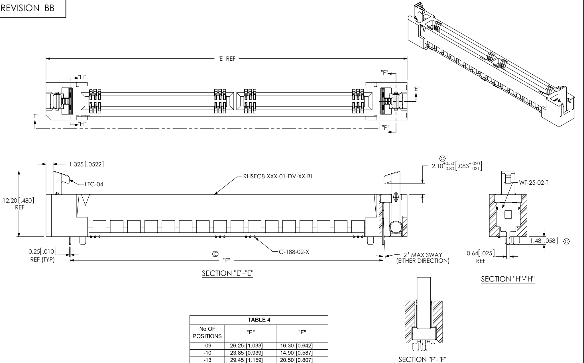
FIG 5 **-BL: BOARD LOCK OPTION HSEC8-160-01-XX-DV-A-BL SHOWN (NOT AVAILABLE FOR -GR TYPE USE) (FOR -09, -13, -25, 37, -40, -49, -50, -60, -70, -80, -90 & -100 POSITIONS DIFFERENT AS SHOWN, OTHERWISE SAME AS FIG 2) (FOR -10, -20 & -30 POSITIONS DIFFERENT AS SHOWN, OTHERWISE SAME AS FIG 1) (** = AVAILABLE ONLY WITH -01 CARD THICKNESS) (SOME FEATURES NOT SHOWN FOR CLARITY) (AVAILABLE IN ALL POSITIONS)
