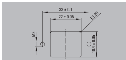
Standardised flange
