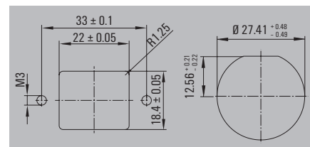
Standardised flange
