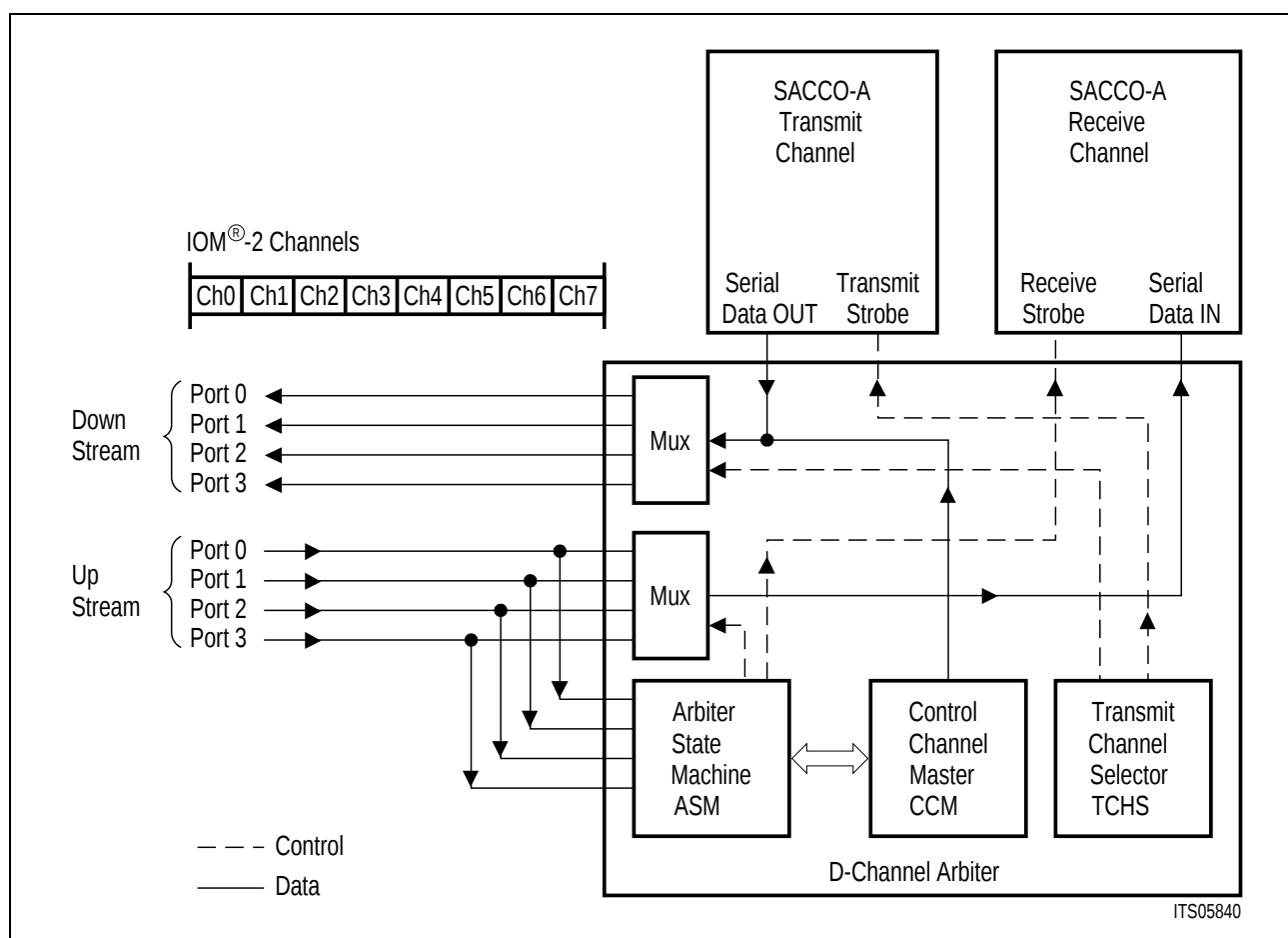
Figure 43 D-Channel Arbiter
