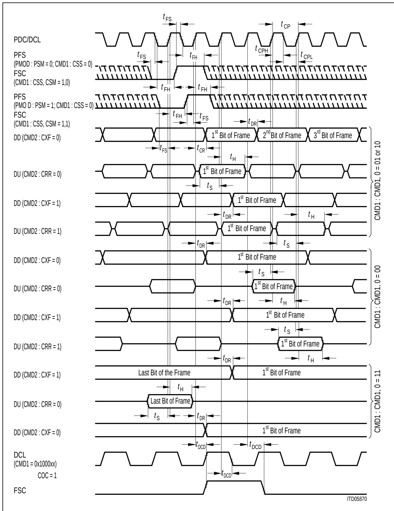
Figure 143 Configurable Interface Timing, CMD:CSP1,0 = 00 (prescaler divisor = 2)
