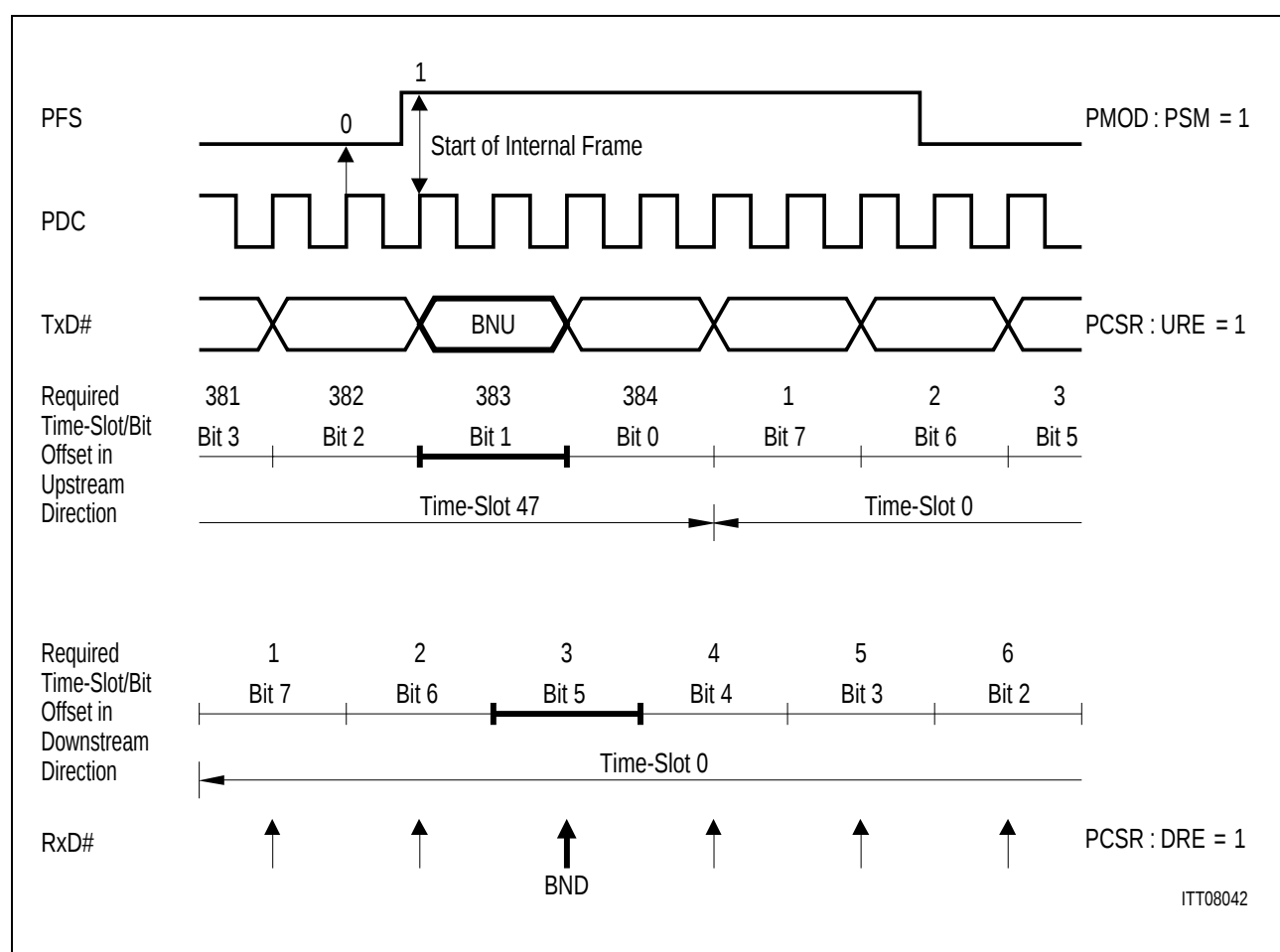
Figure 63 Timing for PCM Frame Offset of Example 2
