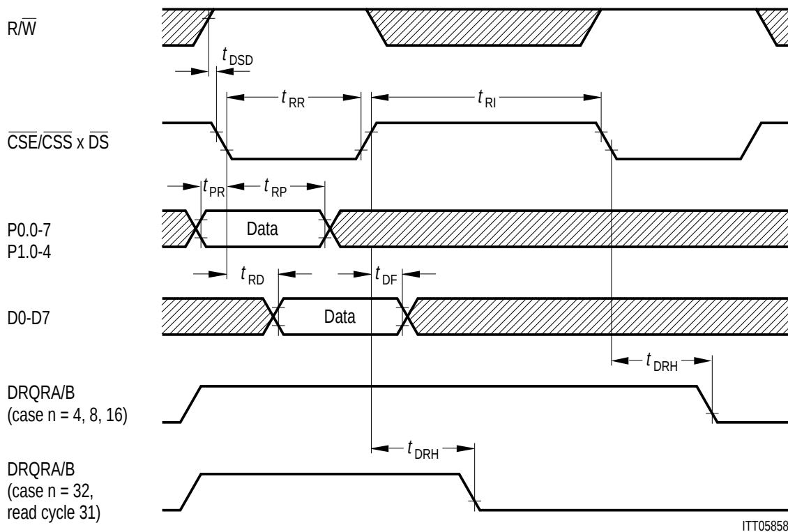
μP Write Cycle
