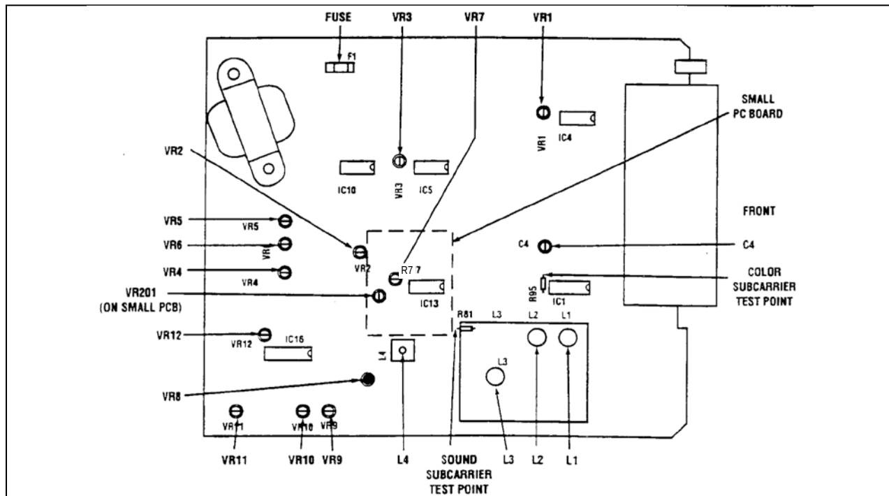
Fig. 8. Adjustment and Test Point Locations.
