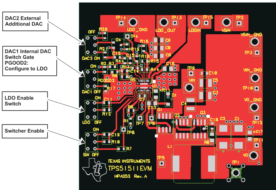
Figure 1-6. Switches and Jumpers
