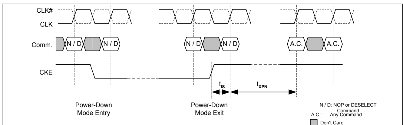
Figure 59 Power-Down Mode
