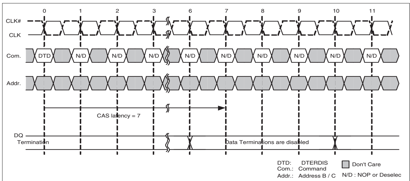
Figure 46 DTERDIS Timing
