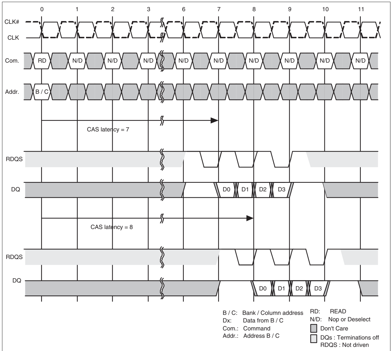
Figure 38 Read Burst
