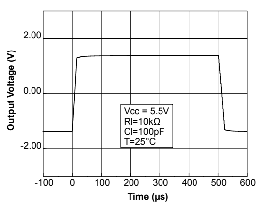
Figure 31. Large signal
