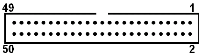
Figure 3.2: Opto-22 CN1/CN2
