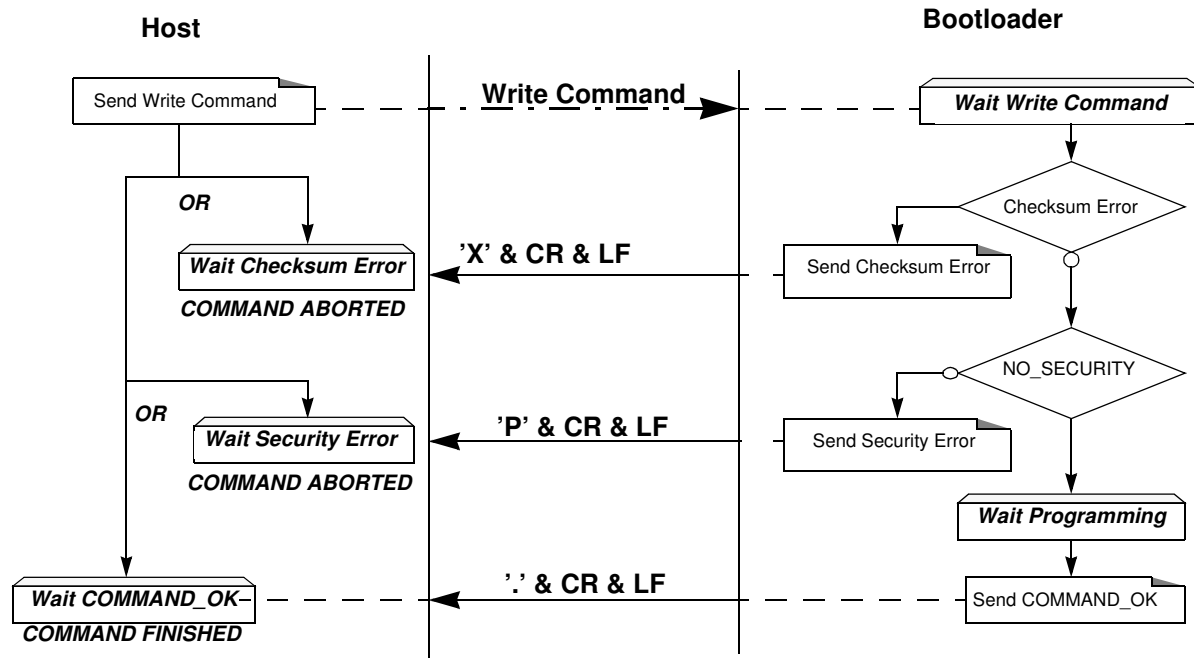
Figure 24-9. Write/Program Flow
