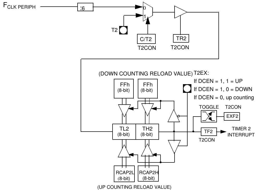
Figure 12-1. Auto-reload Mode Up/Down Counter (DCEN = 1)
