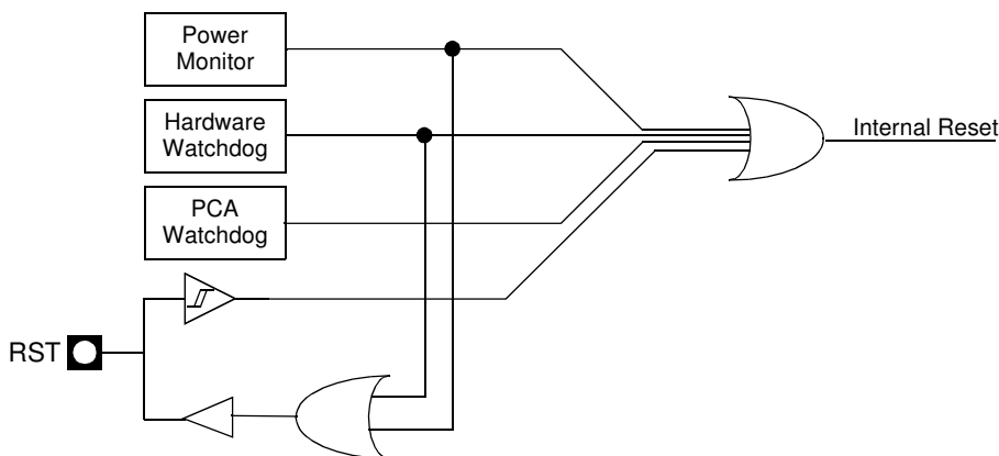
Figure 10-1. Reset schematic
